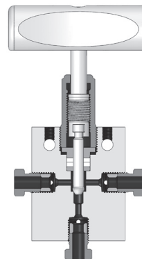
3-Way, 2 Outlet Ports
